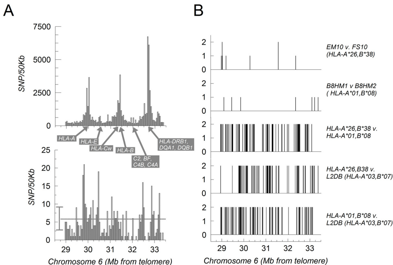
Figure 2 Comparison of SNPs between CEHs. A. Upper panel: Previously reported SNP distribution over the human MHC (NCBI dbSNP Build 126) indicating the higher density of SNPs in the HLA-A, Cw, B and HLA-DR/DQ regions. Across the indicated region (position 28,944,796 to 33,362,643; from ~1 Mb telomeric to HLA-A to ~0.2 Mb centromeric to HLA-DPB1), there is a mean frequency of ~790 SNP/50 kb genomic DNA. Lower panel: Distribution of SNPs incorporated into the Affymetrix GeneChip Human Mapping 500 K array. The horizontal line represents the mean distribution in the region (~5 SNP/50 kb) and the vertical bar to the left of the line indicates one standard deviation. Thus, the chip uses only 0.6% (428 SNPs) of the SNPs reported in the region to date. Note that gene chip SNP representation in the regions harboring defined HLA polymorphic alleles is even lower. B. Top panel: SNP variations were determined between two cell lines (EM10 and FS10) homozygous for the CEH [HLA-A*2601, E*010301, Cw*1203, B*3801, SC21, DRB1*0402, DQA1*0301, DQB1*0302] except for EM10, which is heterozygous for HLA-E*0101 and HLA-E*010301. For all panels in this figure, a value of 0 indicates homozygous identity between the two cell lines, a value of 1 indicates heterozygosity for the SNP in at least one of the cell lines, and a value of 2 indicates complete discordance between the two cell lines. Second panel: SNP variations between the B8HM1 and B8HM2 cell lines each homozygous for the CEH [HLA-A*0101, E*0101, Cw*0701, B*0801, SC01, DRB1*0301, DQB1*0201]. Third panel: A comparison of the homozygous SNP identities shared between EM10 and FS10 (the HLA-A*26, B*38 CEH) cell lines with the homozygous SNP identities shared between B8HM1 and B8HM2 (the HLA-A*01, B*08 CEH) cell lines. Only those SNPs for which there was an unequivocal call for all four cell lines were included. Fourth panel: SNP variations between the HLA-A*26, B*38 CEH and the L2DB cell line homozygous for the independent HLA-A*03, B*07 CEH ([HLA-A*0301, E*010302, Cw*0702, B*0702, SC31, DRB1*1501, DQA1*0102, DQB1*0602]). Bottom panel: SNP variations between the HLA-A*01, B*08 CEH and the L2DB cell line homozygous for the HLA-A*03, B*07 CEH.
