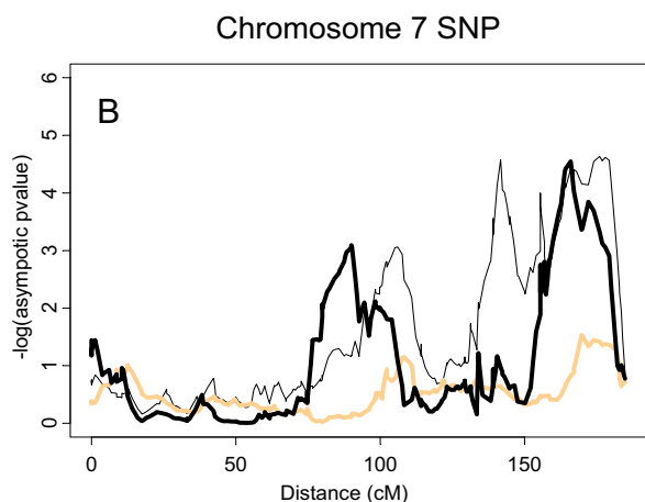
Figure 3 Sib-pair QTL results of P300 amplitude, stratified by smoking status. Linkage results are shown for MS markers (A, N = 735 sib-pairs) and SNPs (B, N = 718 sib-pairs). The negative log of the asymptotic p -value is plotted over distance in cM. Results are shown for the entire group (thin black line), the smoking subgroup (thick tan line), and the non-smoking subgroup (thick black line). Sample sizes in sib-pairs are 228 for MS smoking, 220 for MS non-smoking, 220 for SNP smoking, and 214 for SNP non-smoking groups.
