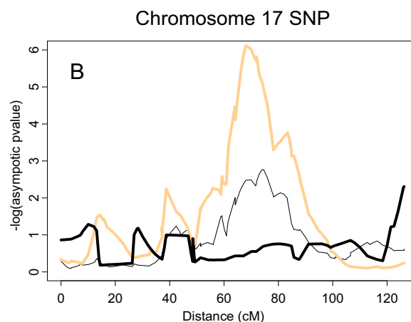
Figure 4 Sib-pair QTL results of P300 amplitude, stratified for alcoholism. Linkage results are shown for MS markers (A, N = 735 sib-pairs) and SNPs (B, N = 718 sib-pairs). The negative log of the asymptotic p -value is plotted over distance in centimorgans (cM). Results are shown for the entire group (thin black line), the alcoholism subgroup (thick tan line), and the non-alcoholism subgroup (thick black line). Sample sizes in sib-pairs are 173 for MS alcoholism, 104 for MS non-alcoholism, 170 for SNP alcoholism, and 103 for SNP non-alcoholism subgroups.
